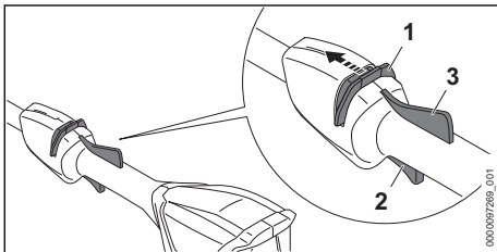
Retaining Latch (1), Trigger Switch (2) and Ergo-Lever (3)
