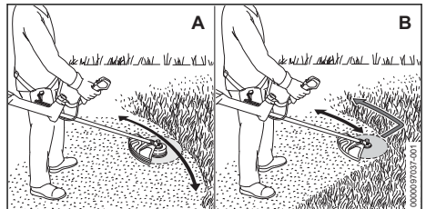
Mowing with a mowing head (A)
